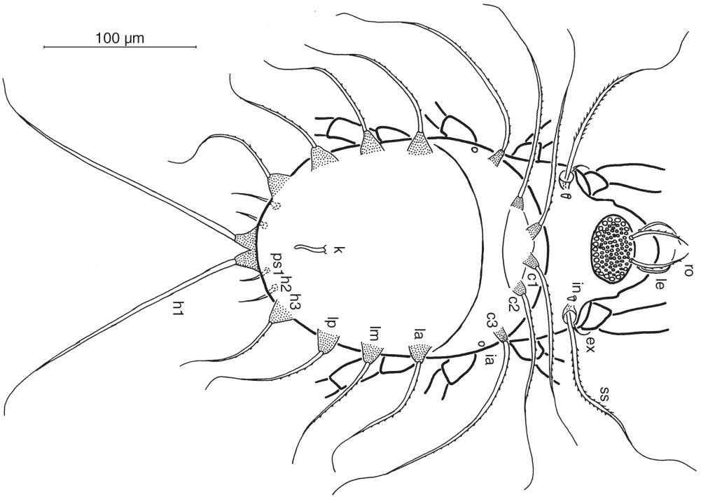
Figure 13. Tokukobelba compia protoyymph, dorsal view.
