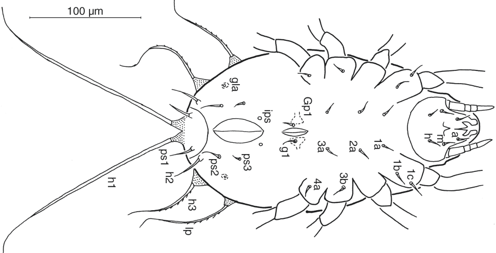
Figure 14. Tokukobelba compia protoyymph, ventral view.
