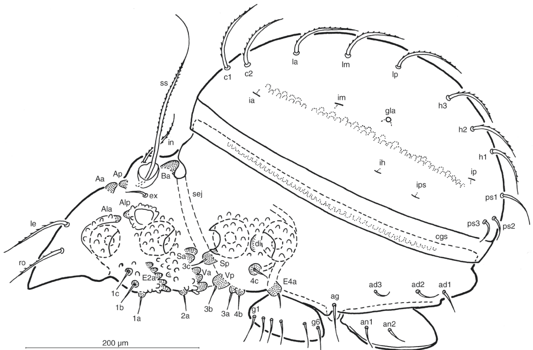
Figure 3. Tokukobelba compta adult, lateral aspect.
